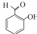
(Salicylaldehyde)
