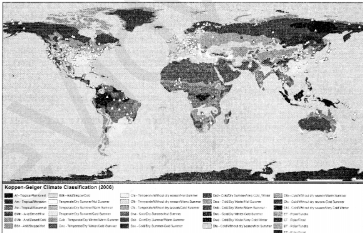
Fig: World map of Köppen-Geiger climate classification
