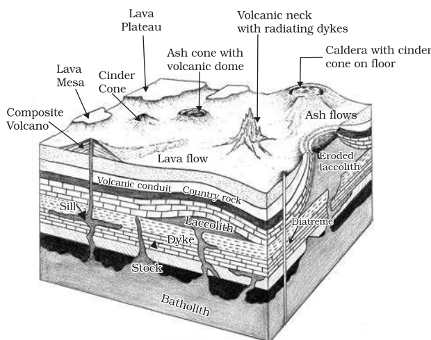
Figure 3.4 : Volcanic Landforms
